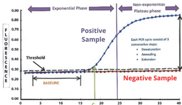
PCR Cycle
